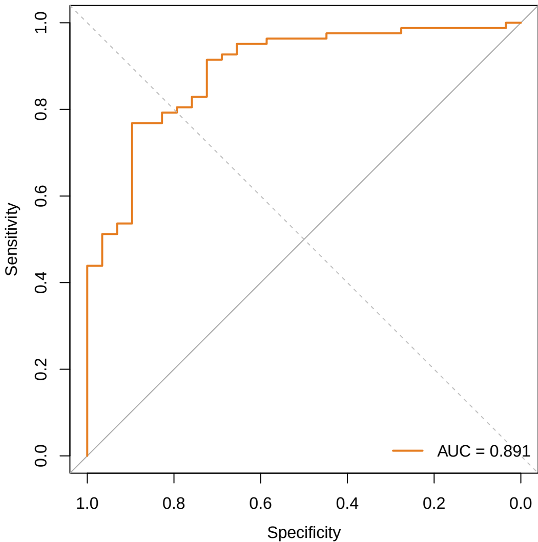
ROC Curve (AUC = 0.891 )
